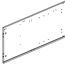
3 (905x400x15mm x1)
