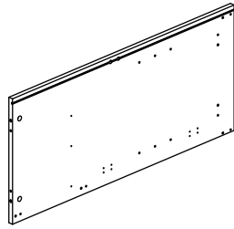
2 (905x400x15mm x1)
