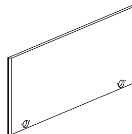
13 (805x380x15mm x1)
