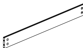
7 (768x80x12mm x1)
