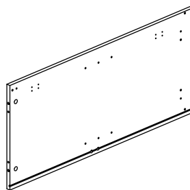
3 (905x400x15mm x1)
