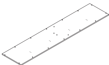
6 (1780*385*15mm x1)
