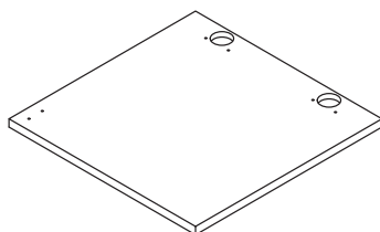
10 (390*390*15mm x1)
