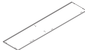
4 (1780*385*15mm x1)
