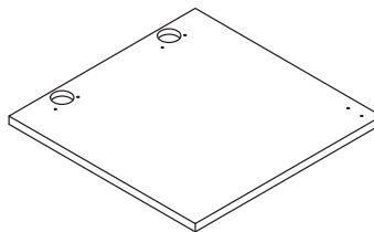
11 (390*390*15mm x1)
