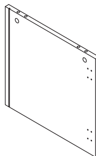
3 (360*384*15mm x1)
