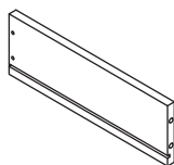
14 (350*115*12mm x2)
