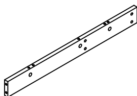
7 (724x75x18mm) X 1
