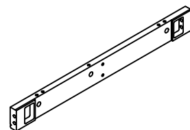
3 (740x75x23mm) X 2
