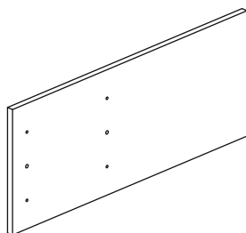
9 (562*235*12mm x2)
