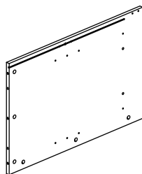
2 (730*475*15mm x1)
