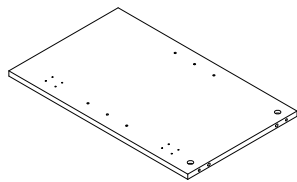
2 (59.1x 36.1x 1.5cm) x1
